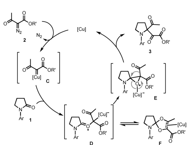
Scheme 2. Mechanistic rationale.
